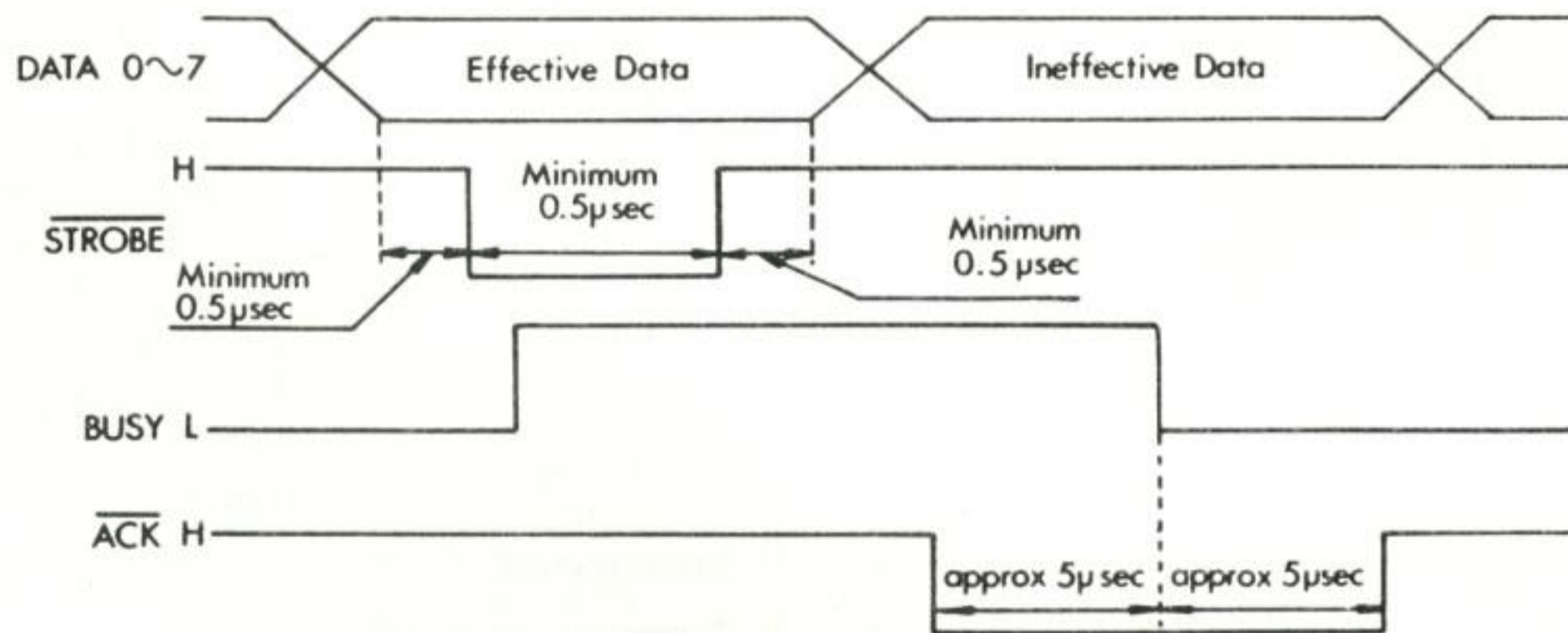
DATA input waveform
